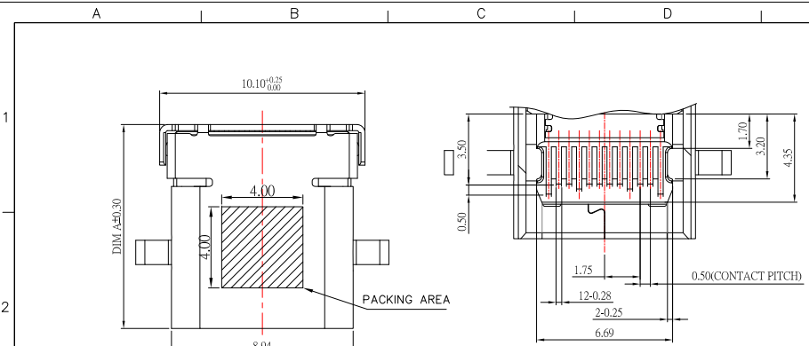
SECTION B-B SCALE 1:1
